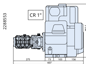
RK 15.15 CR S (Honda engine)
