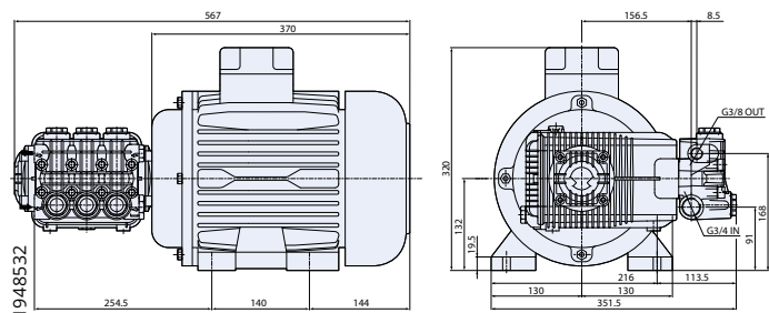
GR. 132 S motor hollow shaft
