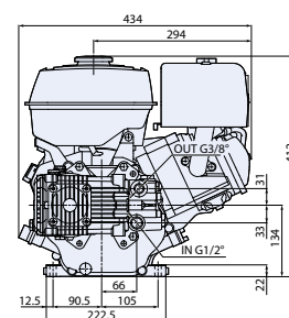
RK CR Honda GX270
